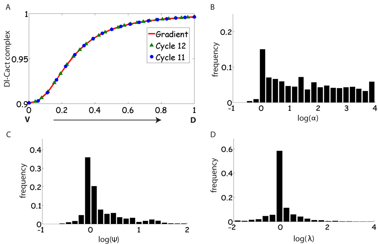
Fig. S1. (A) Illustration of the gradient mapping from cycle 11, with 19 compartments to cycle 12, with 26 compartments. (B–D) Marginal distribution functions for dimensionless rate of Cact degradation (B), stoichiometry (C), and dimensionless transport coefficient (D).
